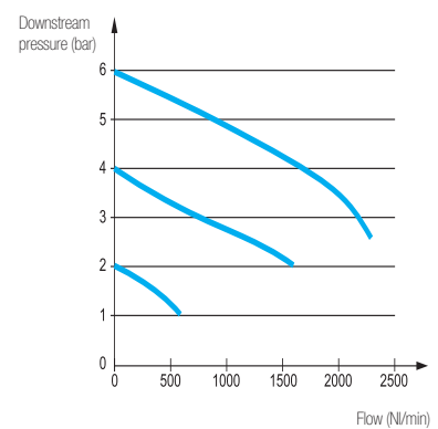
G3/8 Models
