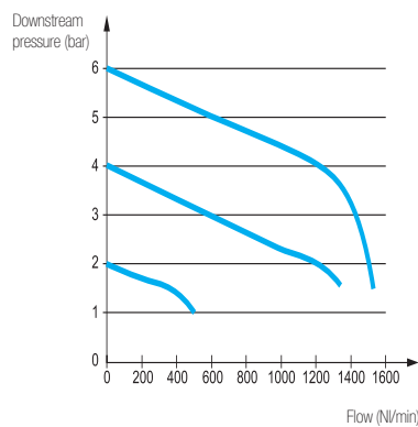
G1/4 Models
